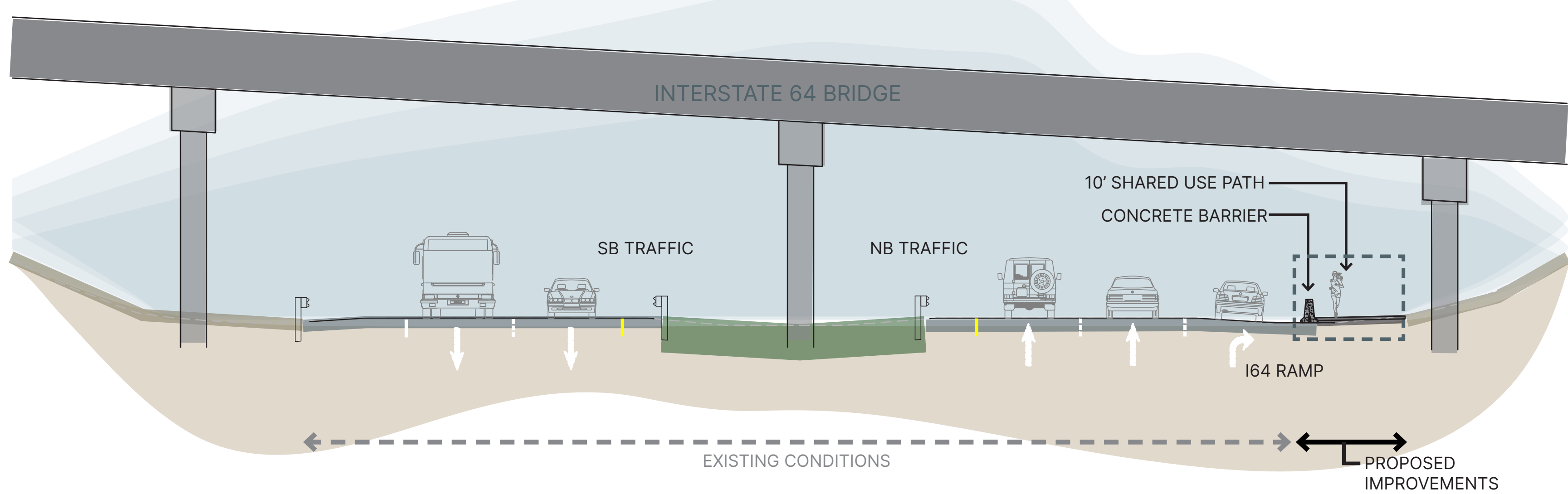
SECTION B
