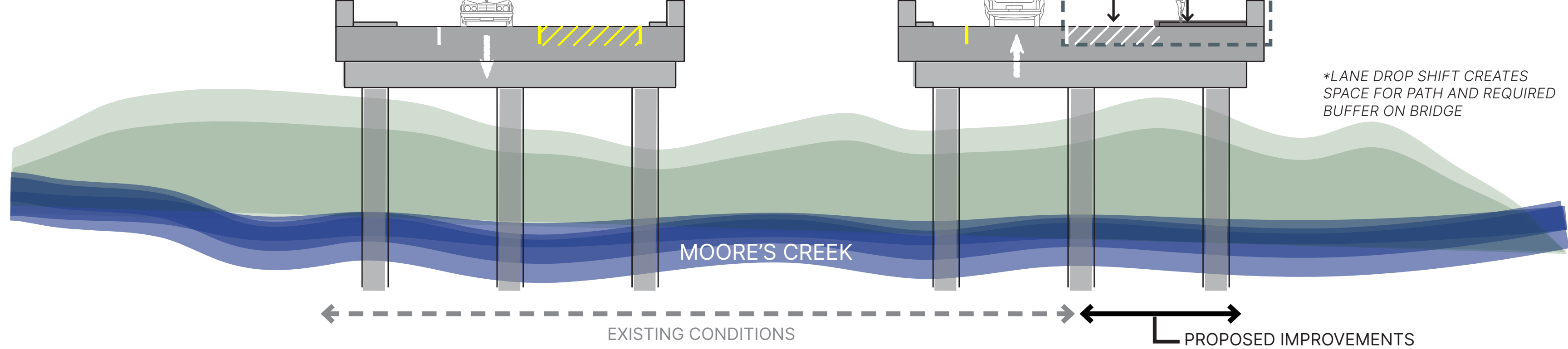
SECTION C
